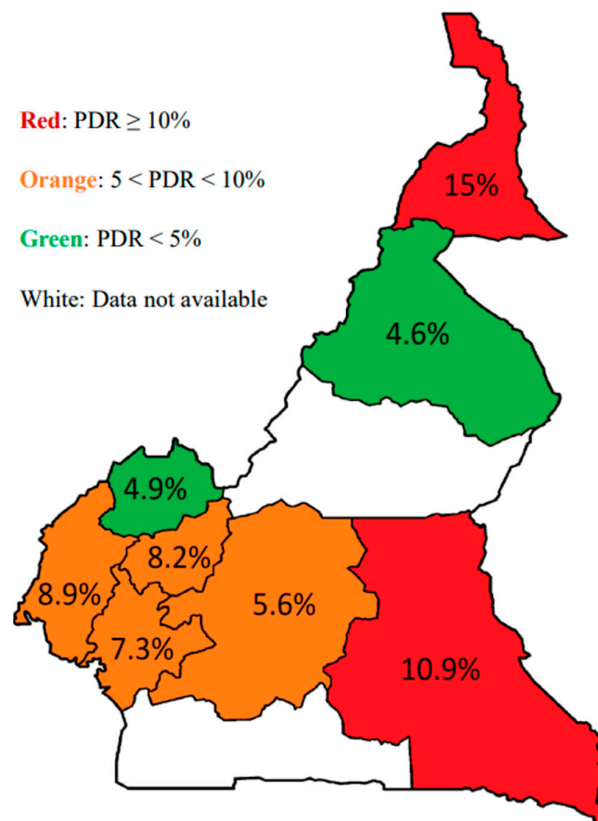
Figure 3. Regional mapping of EFV/NVP-PDR. The figure shows the mapping of EFV/NVP PDR. Red colour denotes regions with high levels of PDR (above the 10% threshold), orange denotes regions with moderate levels of PDR (5–10%), and green denotes regions with levels of PDR below 5%.
