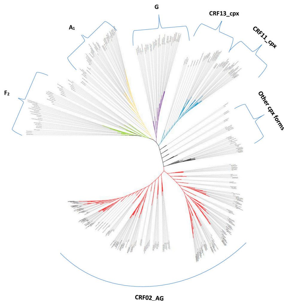
Figure 1. Phylogenetic Tree of HIV-1 sequences from ART-naïve individuals. The evolutionary history was inferred by using the Maximum Likelihood method and Tamura-Nei model [1]. The tree with the highest log likelihood (−69,062.29) is shown. Initial tree(s) for the heuristic search were obtained automatically by applying Neighbor-Join and BioNJ algorithms to a matrix of pairwise distances estimated using the Tamura-Nei model and then selecting the topology with superior log. Cpx = complex recombinant forms.
